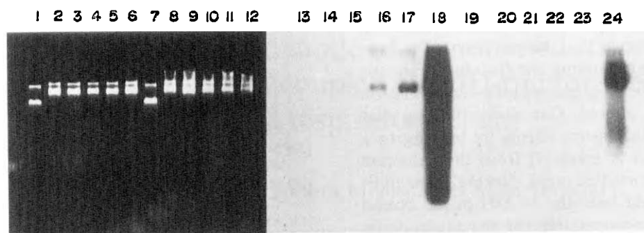
Fig. 2. Gel mobility retardation and ternary complex analysis of pAR1539 (T7A2) with RNA polymerase and NTPs. The control plasmid DNA (20 nM, lanes 1 and 7) was treated at 37°C for 10 min with E. coli RNA polymerase (200 nM) in the absence of any NTP (lane 2), in the presence of (lane 3) GTP alone, (lane 4) GTP and CTP, (lane 5) GTP, CTP and UTP, and (lane 6) all four NTPs. Lanes 8–12 are the same as lanes 2–6, respectively, except that these were incubated with 100 μM rifampicin at 37°C for 5 min prior to loading. The concentration of GTP was 200 μM, while the other NTPs were used at 10 μM; [ \alpha - 32 P]-CTP was at 2 μCi/nmol. Samples were analyzed over a 1% agarose gel in Tris-borate-EDTA buffer (pH 8.3) at 1.5 V/cm for 6 h. Lanes 13–24 represent the same samples as lane 1–12, respectively, when dried and autoradiographed.
